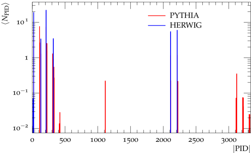
Average per-event multiplicity of decayed particle IDs
